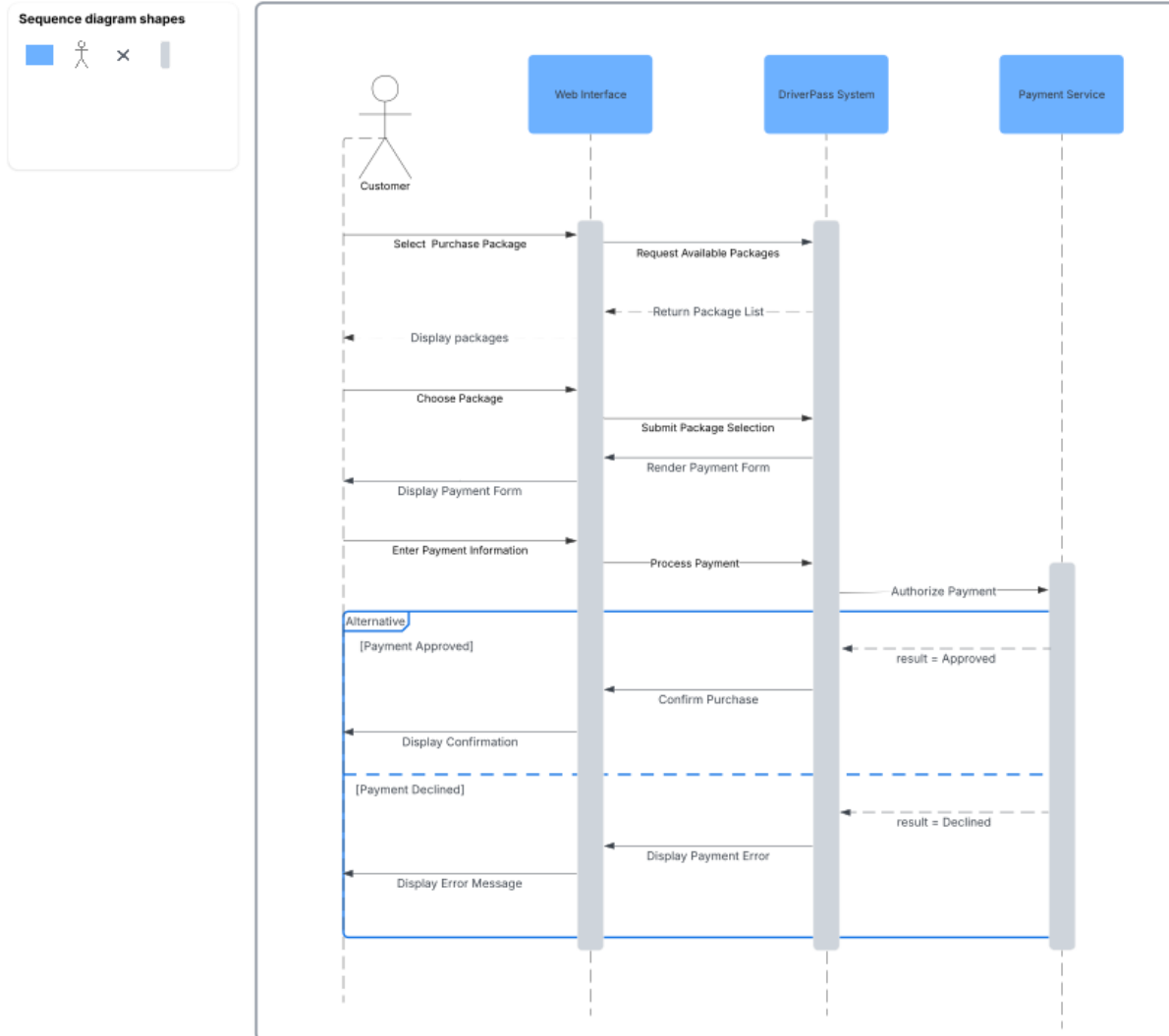
Purchase Package Sequence Diagram
